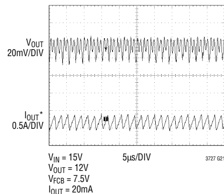
Constant Frequency (Burst Inhibit) Operation (Figure 12)
