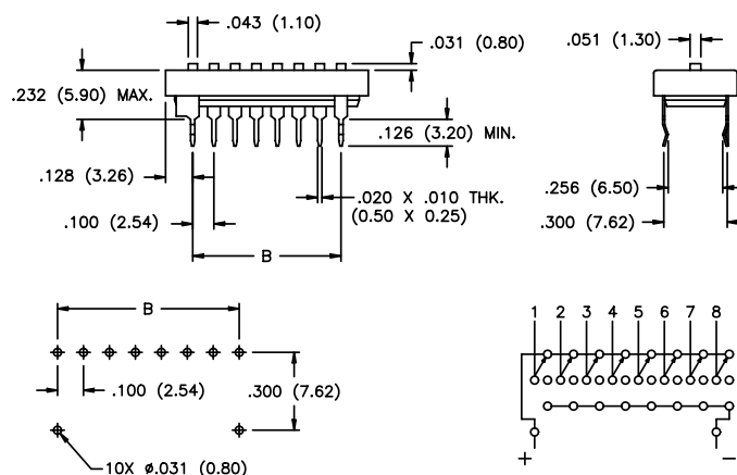
PRINTED CIRCUIT BOARD OUTLINE (8 POSITIONS SHOWN)
