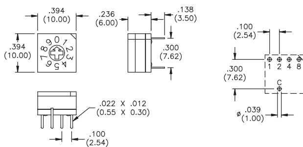
Mechanical outline
