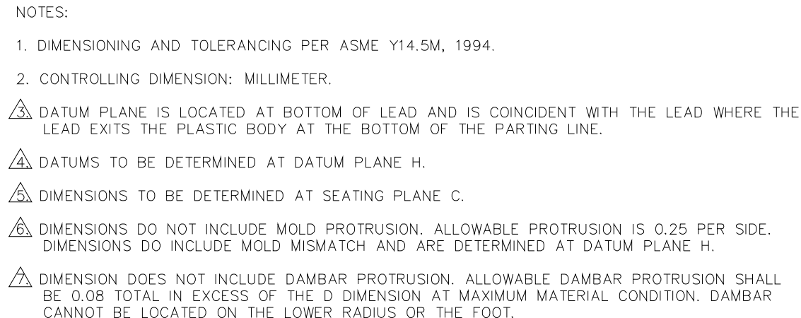
Figure 8. MCF5208CAB166 Package Dimensions (Sheet 2 of 2)
