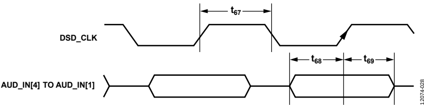
Figure 26. DSD Timing
