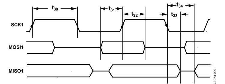
Figure 8. Serial Port 1 Slave Mode Timing (SPI Mode 0 and SPI Mode 3)
