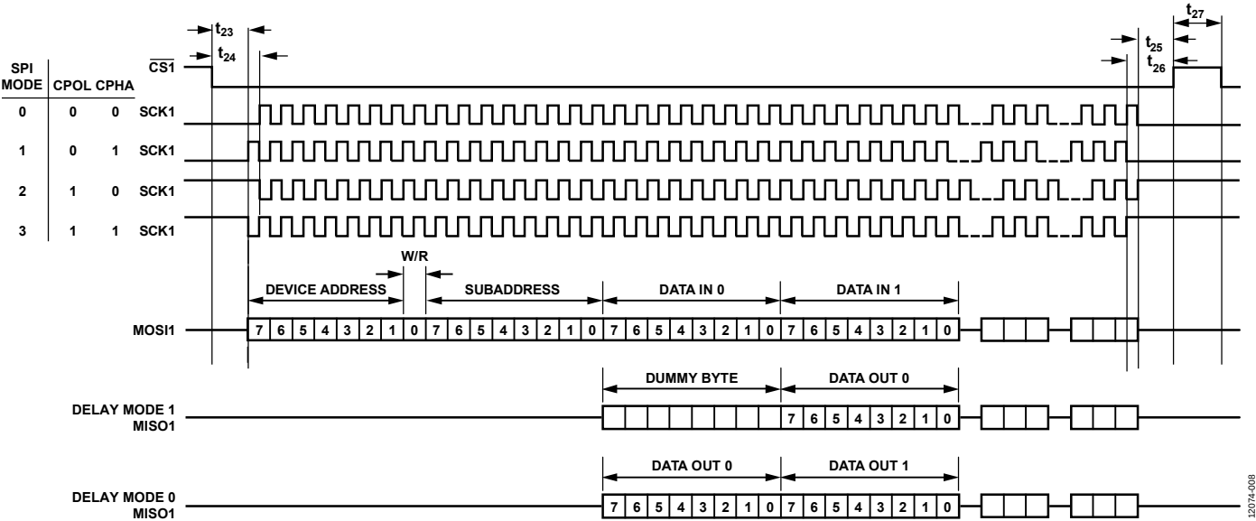
Figure 7. Detailed SPI Slave Timing Diagram (Serial Port 1)
