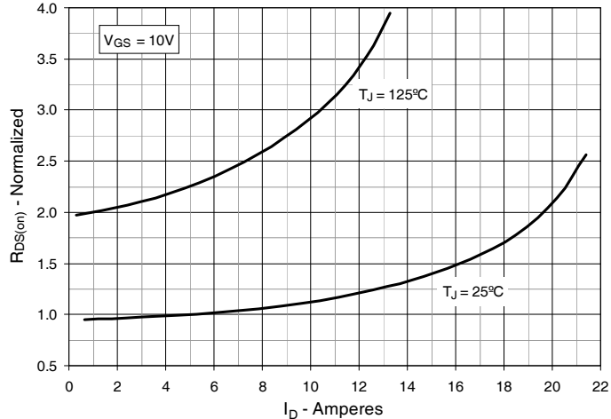
Fig. 5. R_{DS(on)} Normalized to I_D = 6\text{A} Value vs. Drain Current
