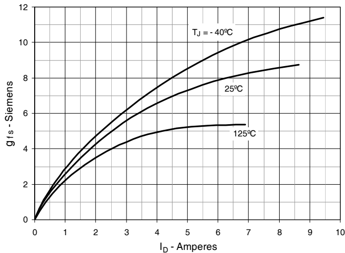
Fig. 9. Transconductance
