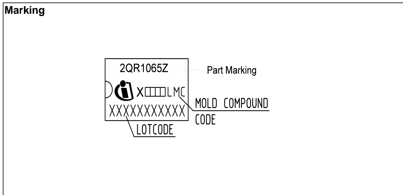
Figure 15 Marking for ICE2QR1065Z
