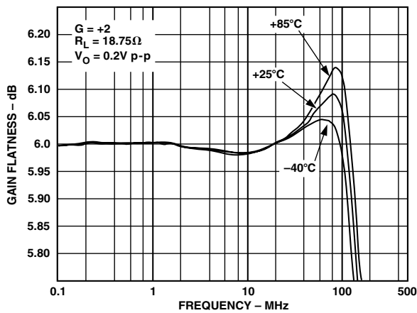
Figure 5. Gain Flatness vs. Frequency Over Temperature (−40°C to +85°C)
