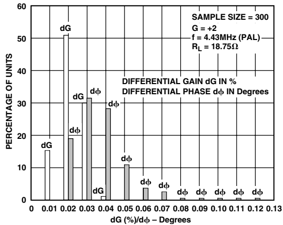
Figure 3. Distribution of Differential Gain (dG) and Differential Phase (dφ); R L = 18.75 Ω
