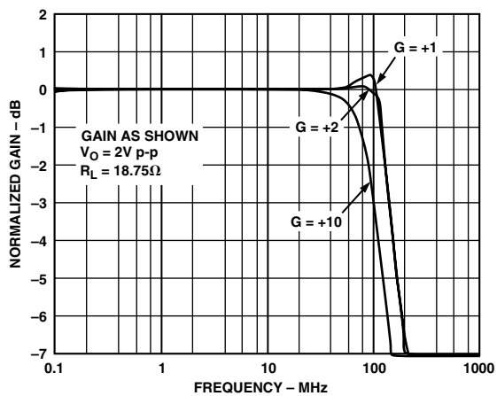
Figure 17. Large Signal Frequency Response; V_O = 2 \text{ V p-p}
