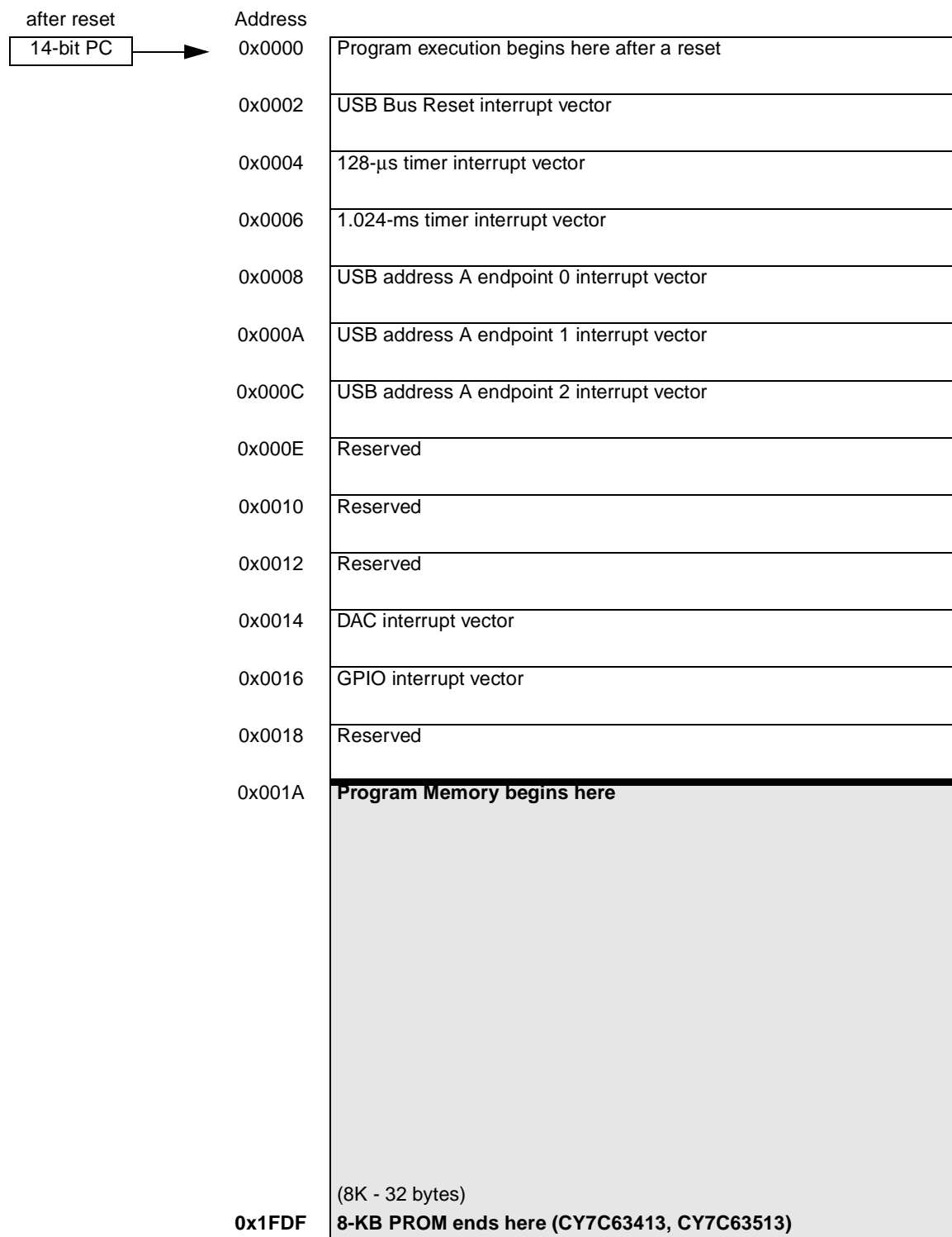
Figure 6-1. Program Memory Space with Interrupt Vector Table
