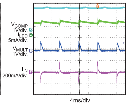
Triac Dimming
