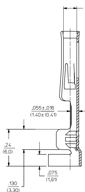
SECT. "C-C"
