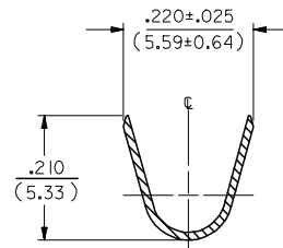
SECT. "A-A"
