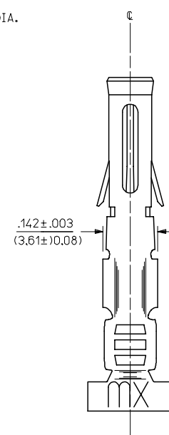
SECT. "B-B"
