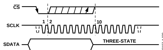
Figure 30. Entering Power-Down Mode
