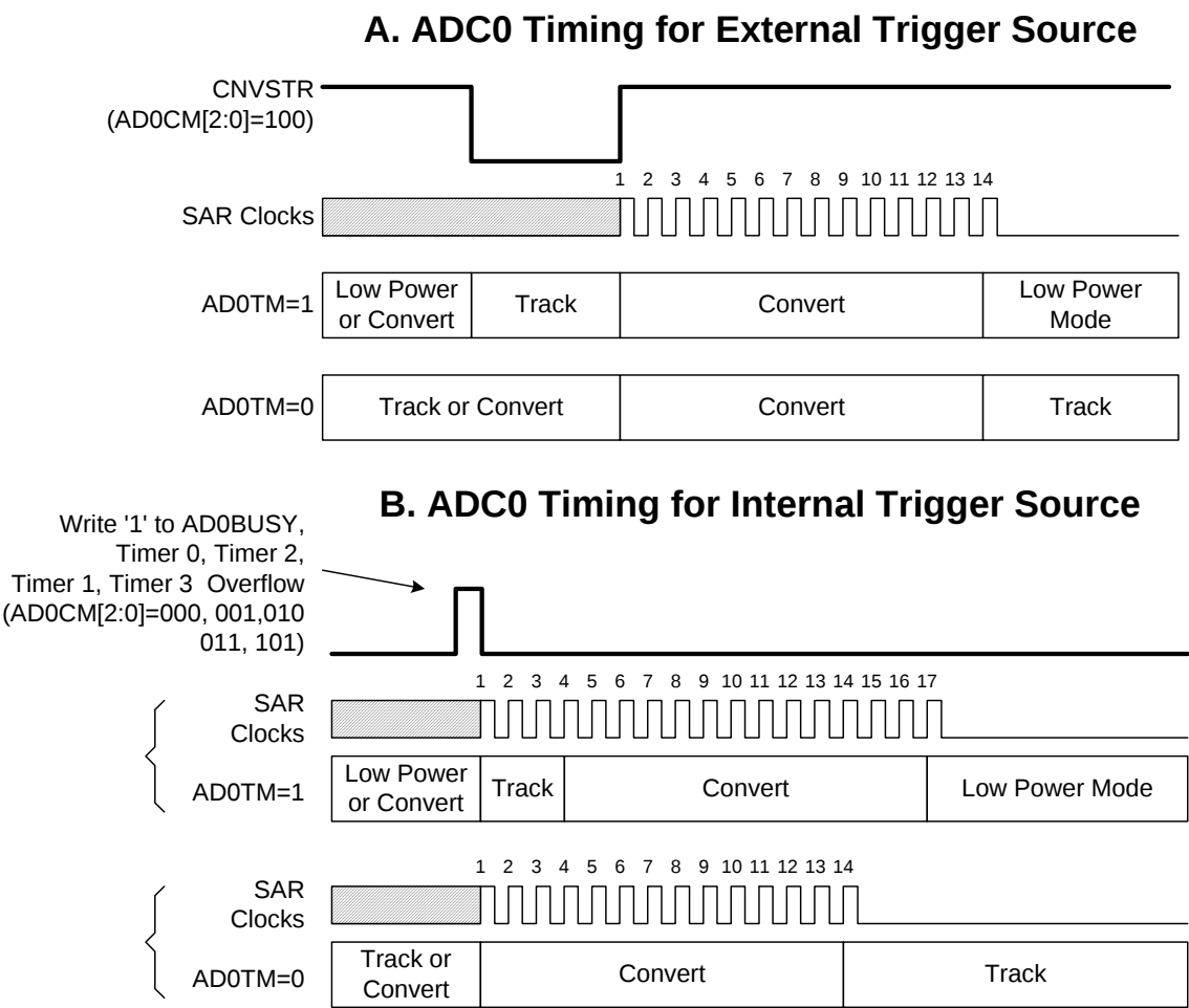
Figure 7.2. 10-Bit ADC Track and Conversion Example Timing
