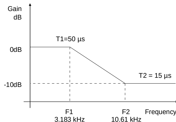
Figure 7. De-Emphasis Curve
