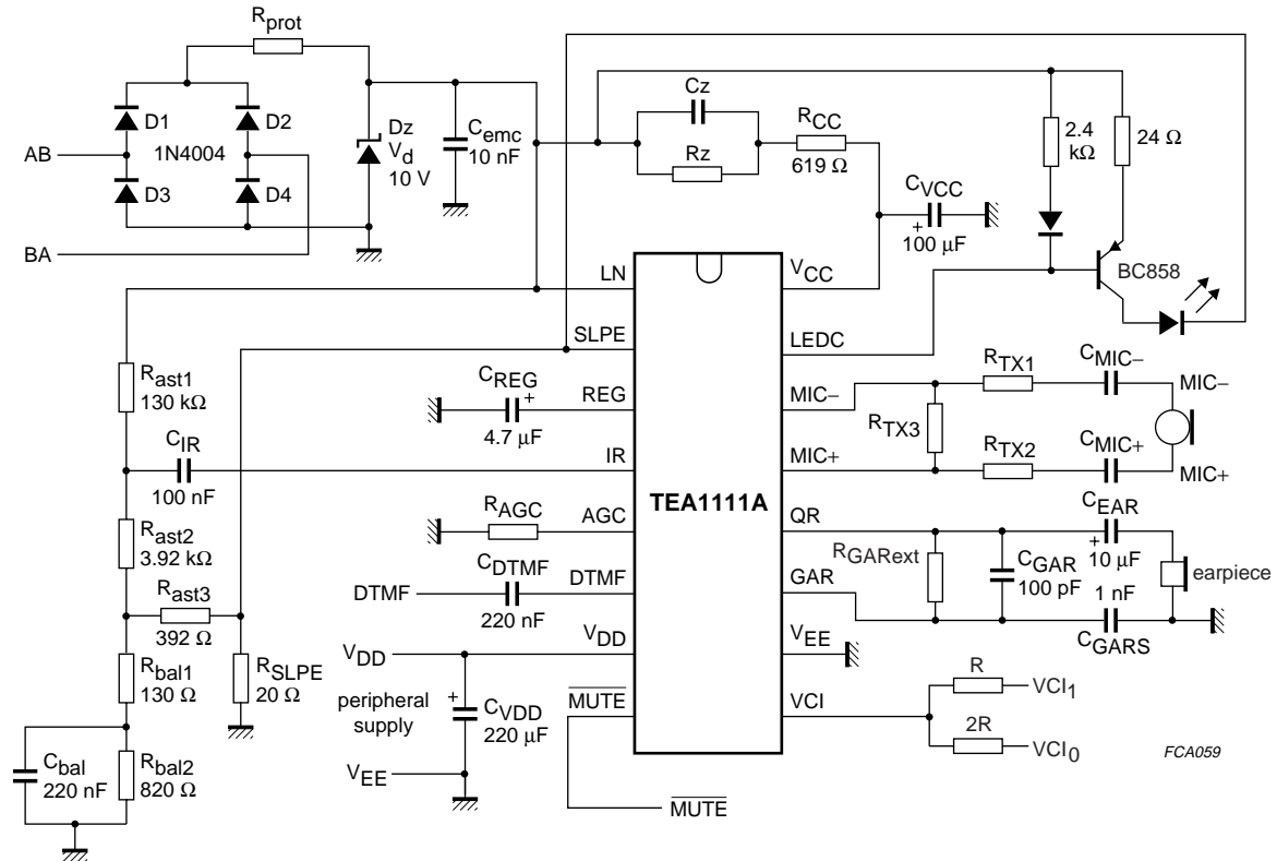
Fig.13 Basic application diagram.
