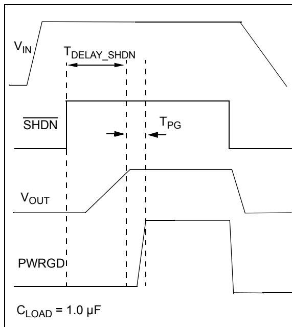
FIGURE 4-3: Power Good Timing from Shutdown.
