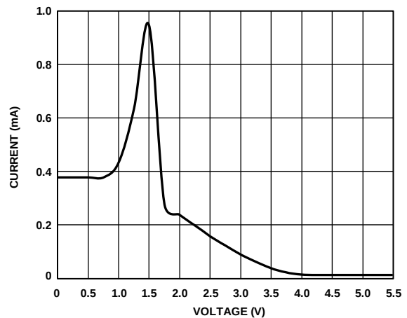
Figure 24. Supply Current I_{DD} vs. Digital Input Voltage
