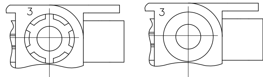
DETAIL A OPTIONAL CONSTRUCTION
