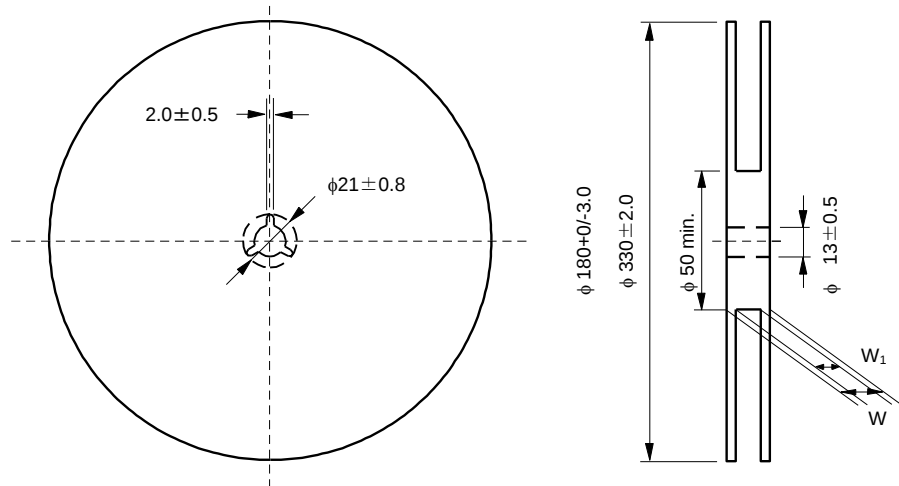
Fig.3 Taping Diagram
