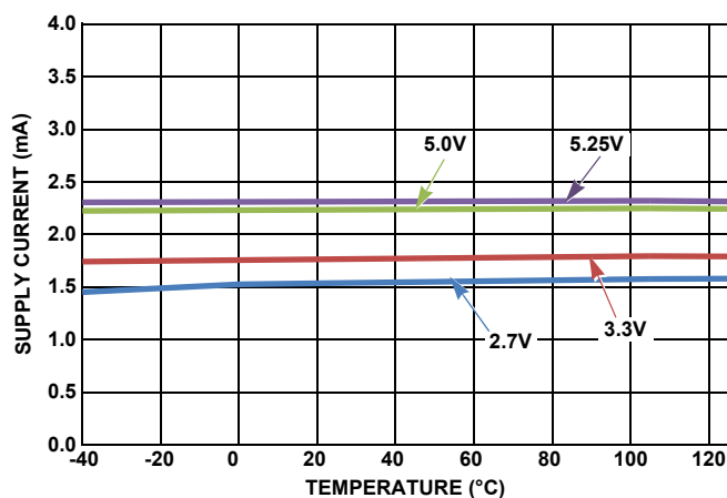
FIGURE 10. SUPPLY CURRENT vs VOLTAGE AND TEMPERATURE
