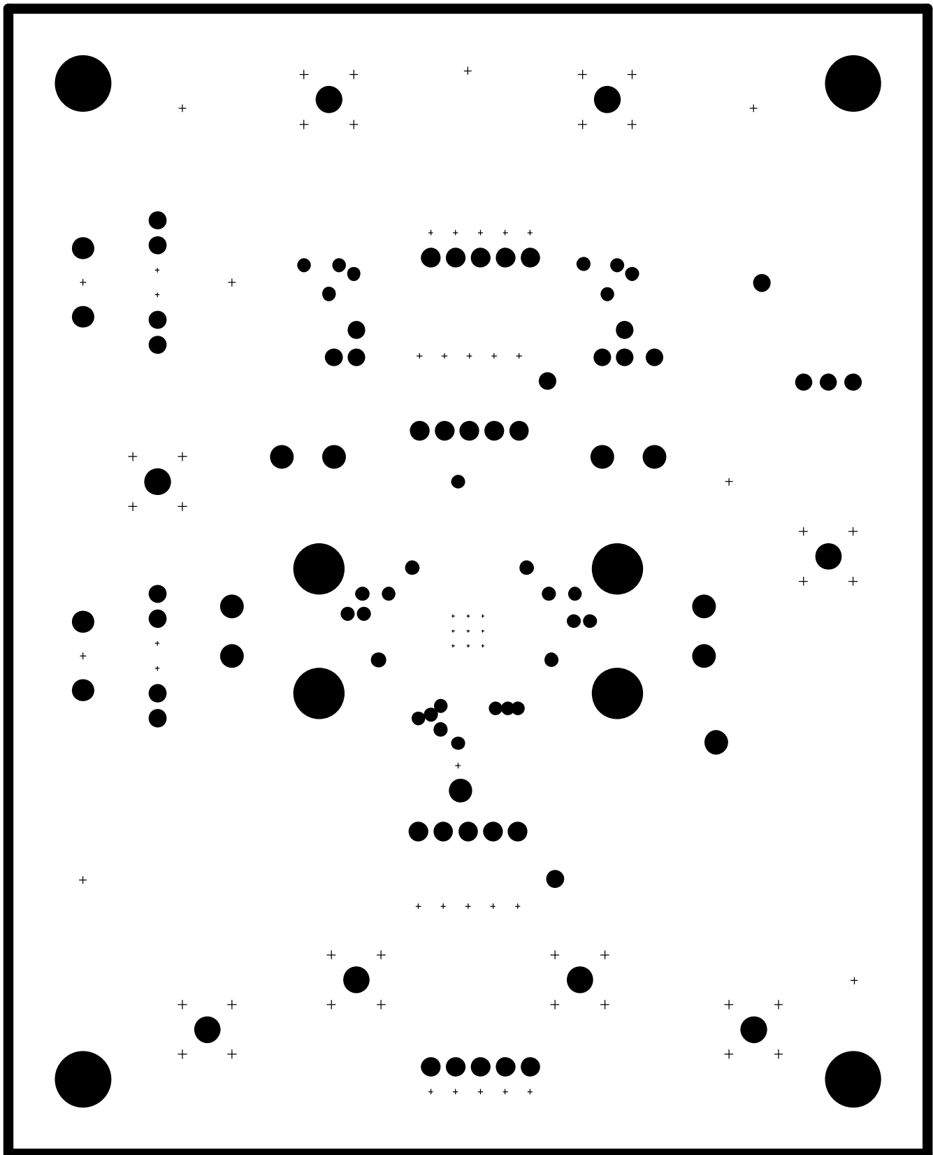
Figure 4. VCA2615EVM PCB Ground Layer (Top View)
