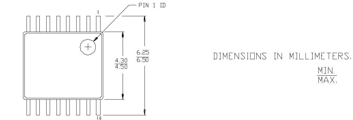
16-lead Thin Shrunk Small Outline Package (4.40 MM Body) Z16
