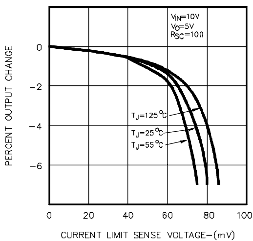
FIGURE 3. CURRENT LIMITING
