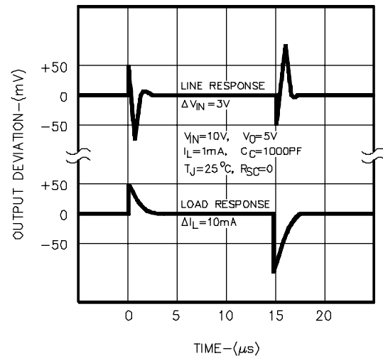
FIGURE 6. TRANSIENT RESPONSE
