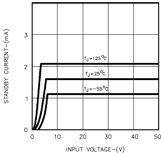
FIGURE 1. STANDBY CURRENT
