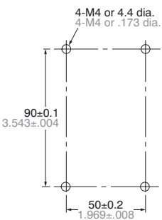
Mounting dimensions
