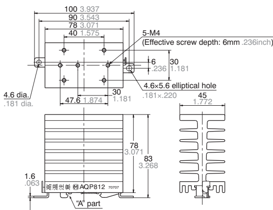
External dimensions
