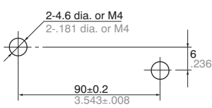
Mounting dimensions (Top view)
