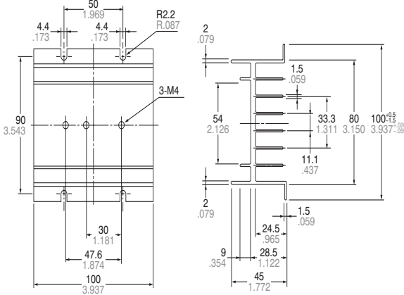
External dimensions
