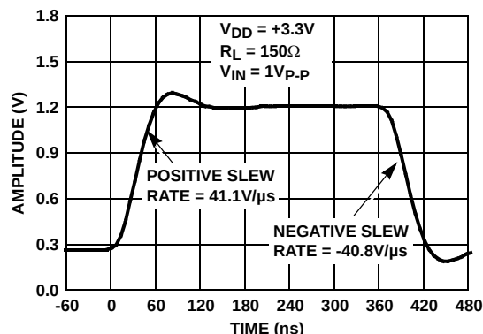
FIGURE 12. SLEW RATE
