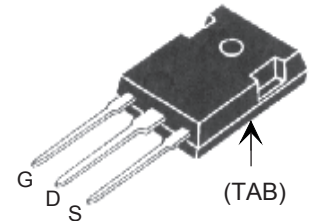
TO-247 (IXTH)
