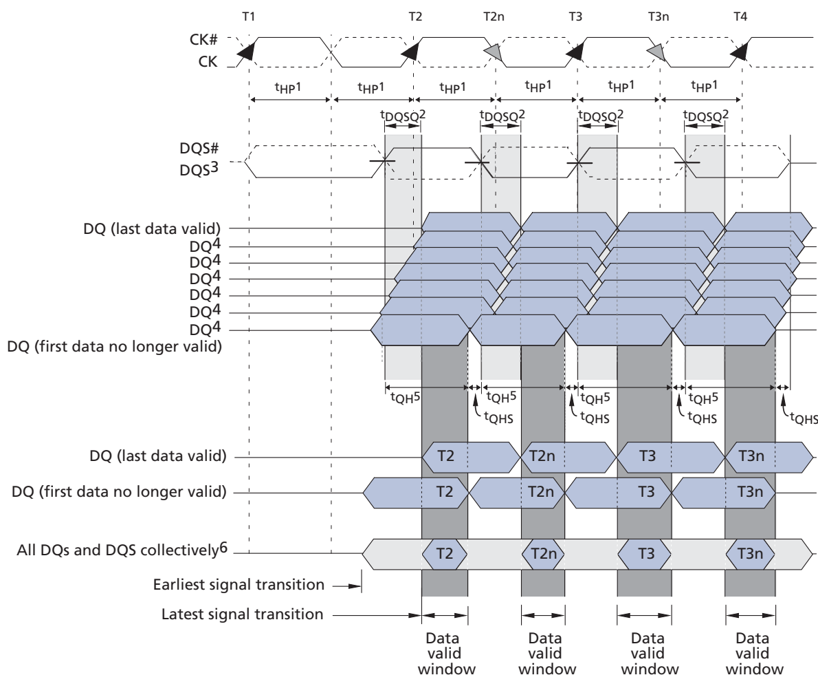
Figure 54: x8 Data Output Timing – t_{DQSQ} , t_{QH} , and Data Valid Window
