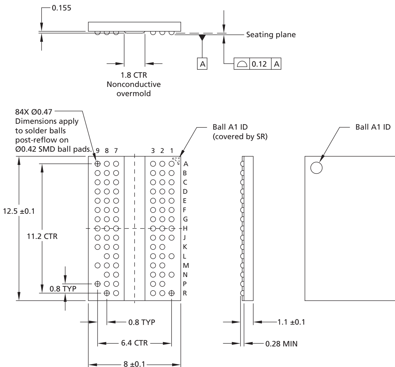
Figure 9: 84-Ball FBGA (8mm x 12.5mm) – x16; "NF" Die Rev :H
