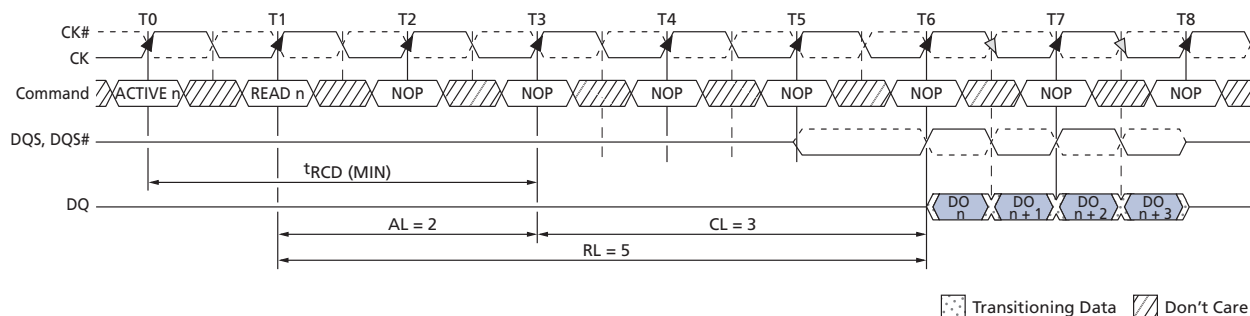
Figure 38: READ Latency
