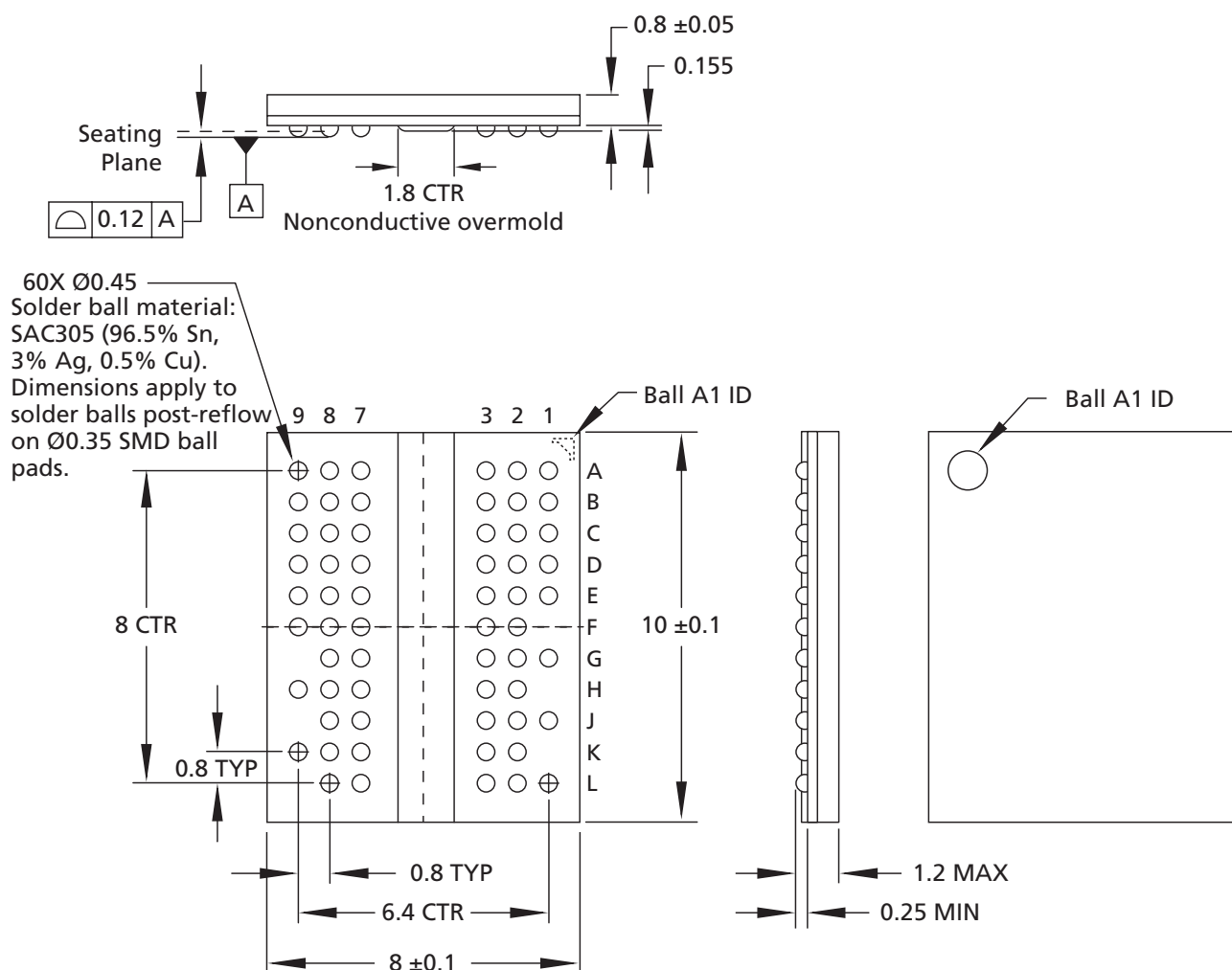
Figure 8: 60-Ball FBGA (8mm x 10mm) – x8; Die Rev :G
