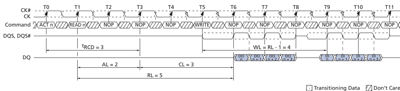
Figure 49: READ-to-WRITE
