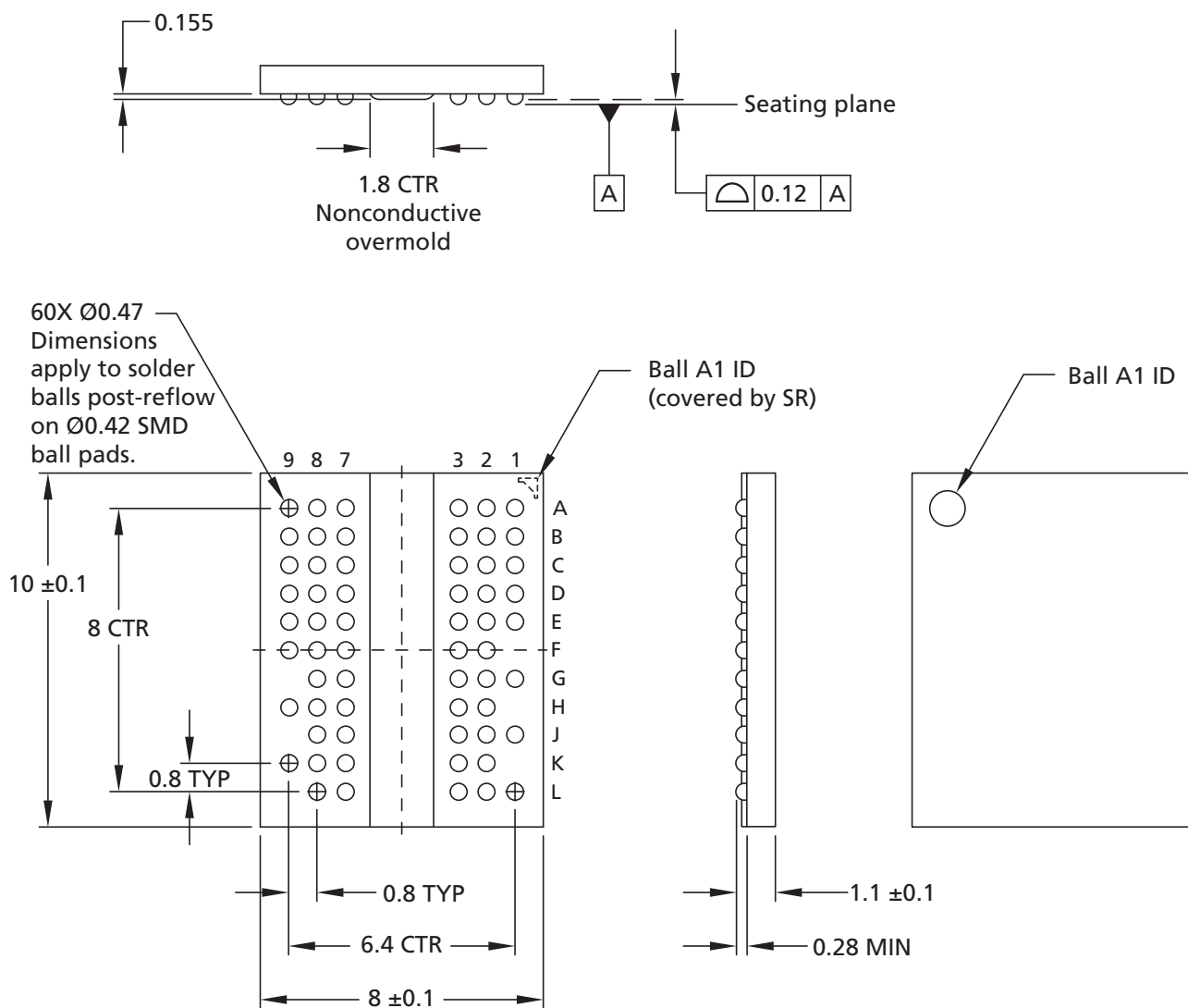
Figure 10: 60-Ball FBGA (8mm x 10mm) – x8; "SH" Die Rev :H
