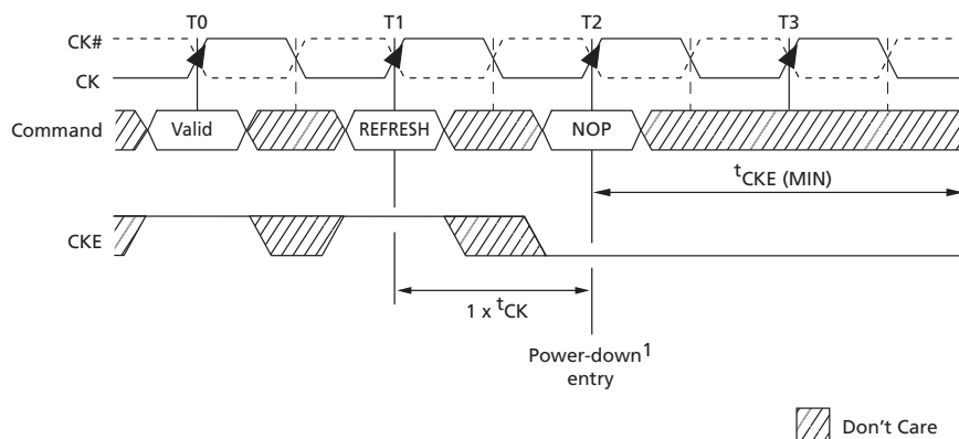
Figure 74: REFRESH Command-to-Power-Down Entry
