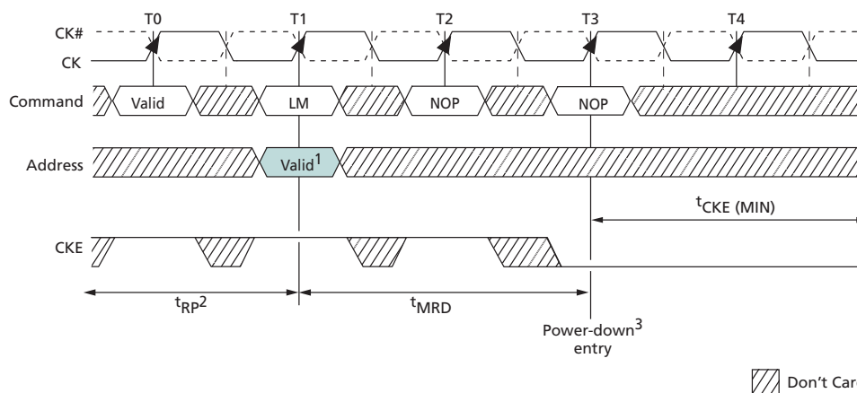
Figure 77: LOAD MODE Command-to-Power-Down Entry
