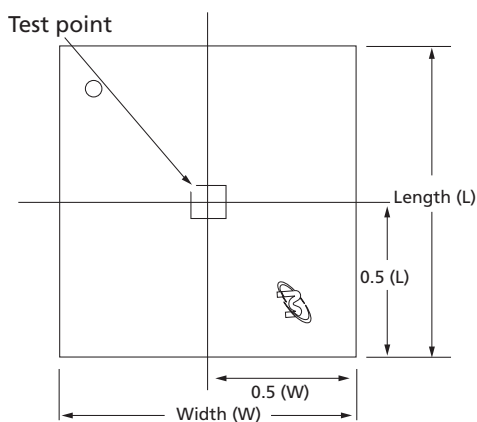
Figure 11: Example Temperature Test Point Location
