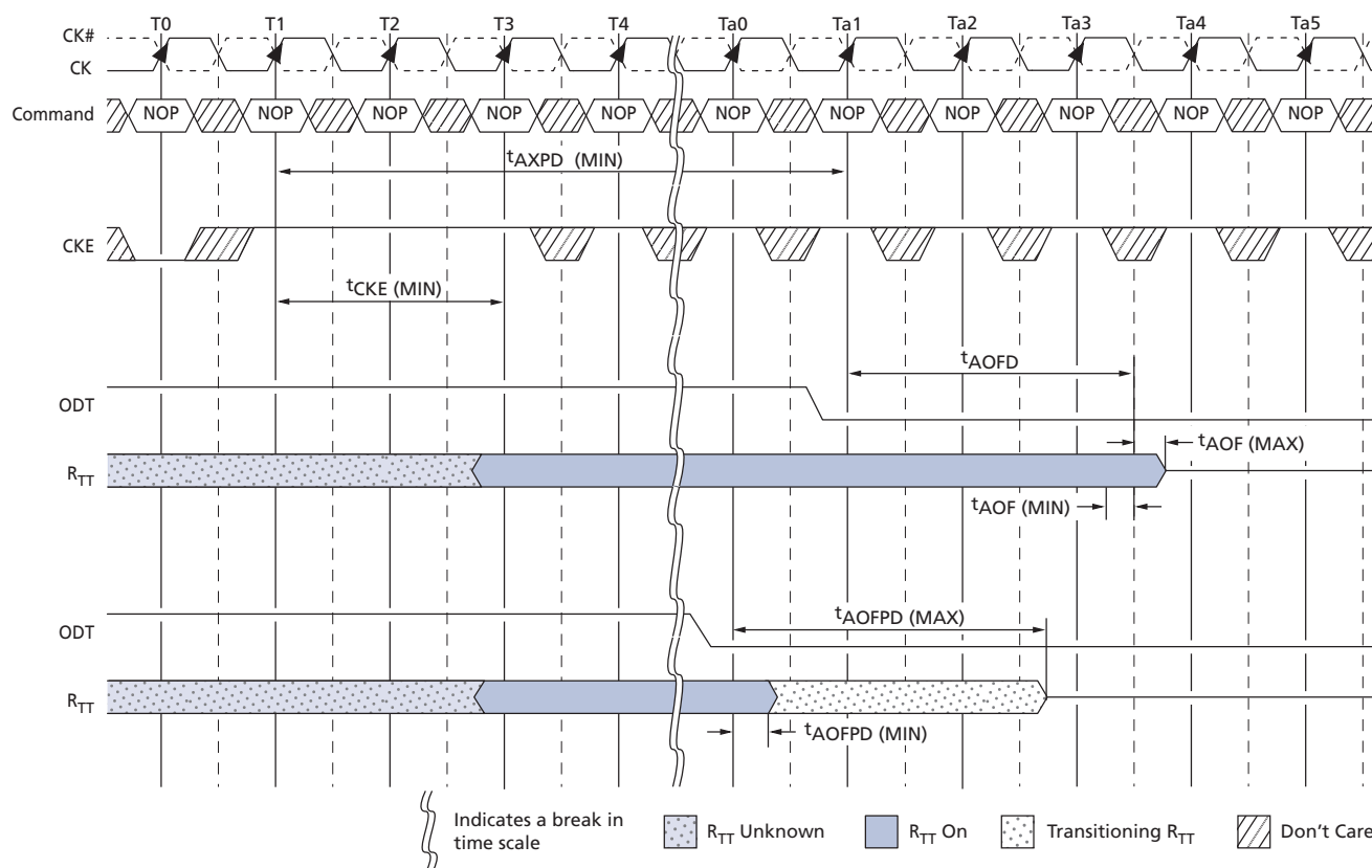
Figure 86: ODT Turn-Off Timing When Exiting Power-Down Mode
