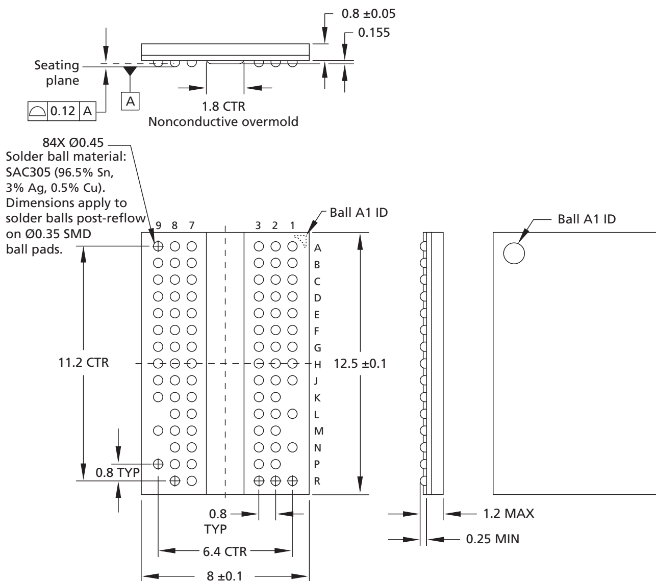
Figure 7: 84-Ball FBGA (8mm x 12.5mm) – x16; Die Rev :G
