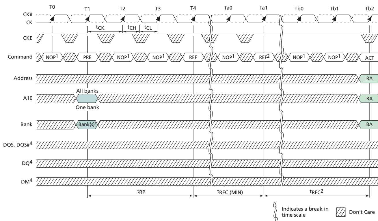
Figure 67: Refresh Mode
