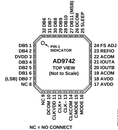
Figure 4. 32-Lead LFCSP Pin Configuration
