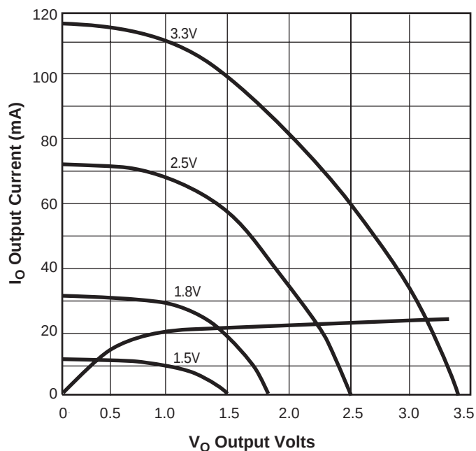
Figure 4: Typical I/O Output Curves
