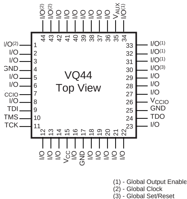
Figure 6: VQ44 Package
