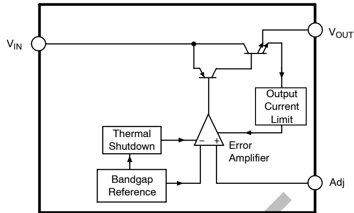
Figure 2. Block Diagram
