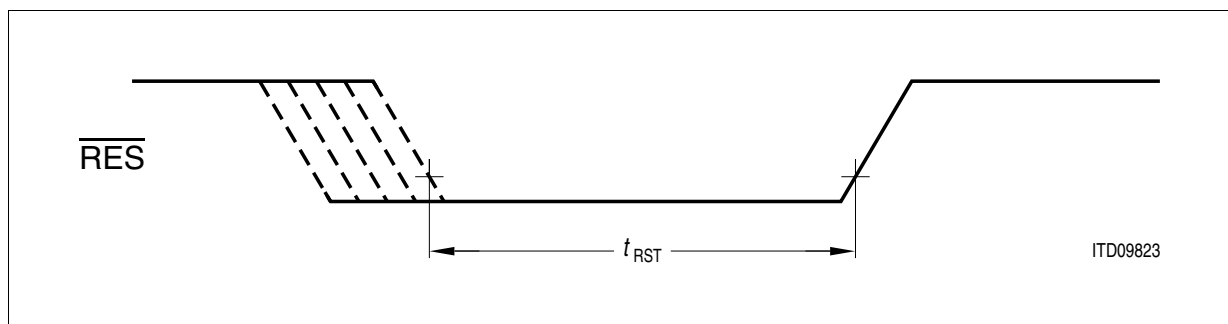
Figure 94 External Reset Timing
