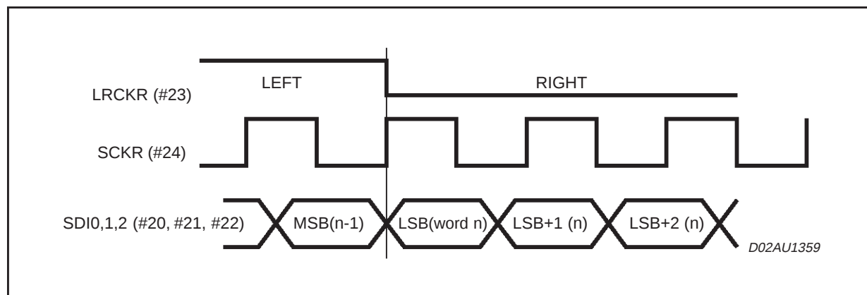
Figure 4. SAI protocol when RLRS=0; RREL=0; RCKP=0; RDIR=0.
