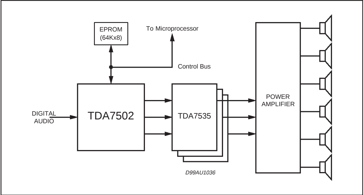
Figure 14. Block Diagram of Car Amplifier Audio Sub-System.
