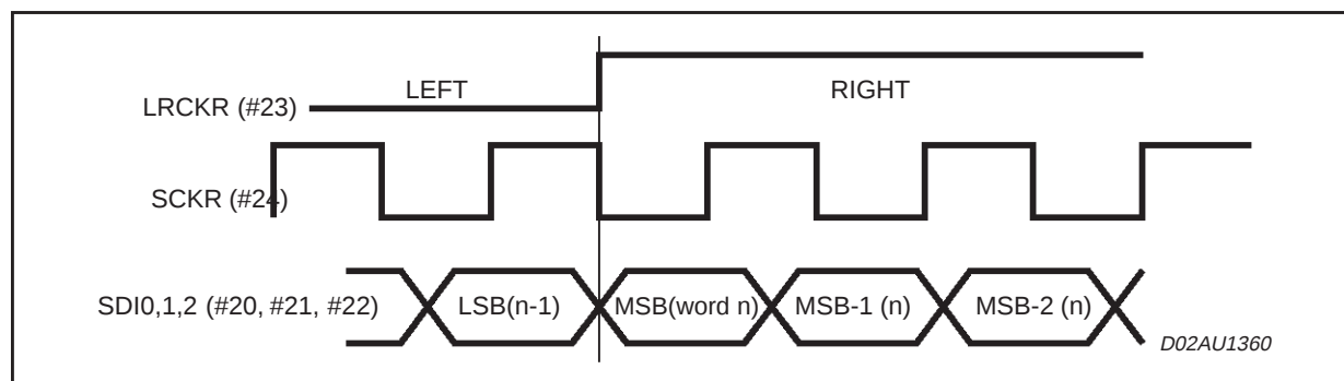
Figure 5. SAI protocol when RLRS=0; RREL=1; RCKP=1; RDIR=0.
