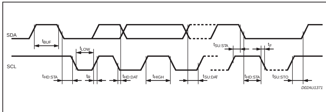
Figure 12. Definition of Timing for the I 2 C BUS.
