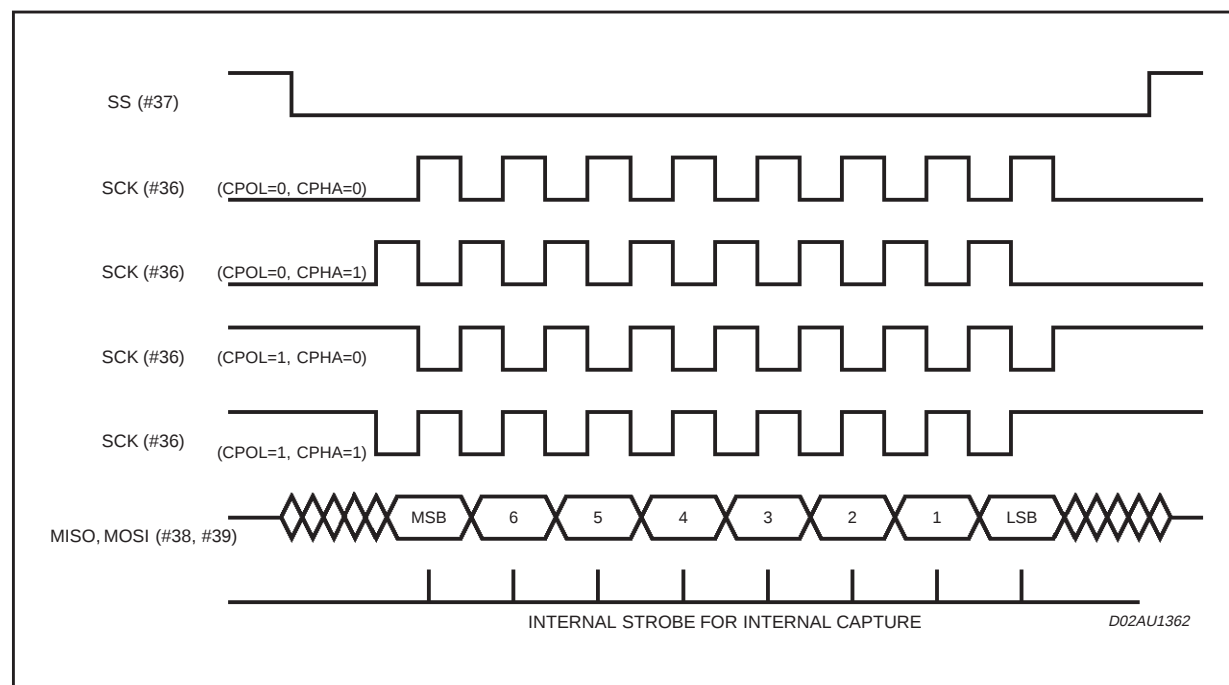
Figure 6. SPI Clocking scheme.
