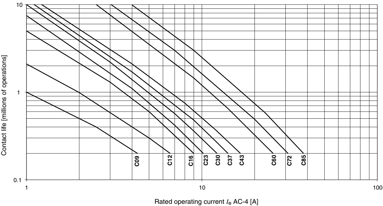
AC-4 Stepping of squirrel-cage motors; U_e = 230...690\text{ V}
