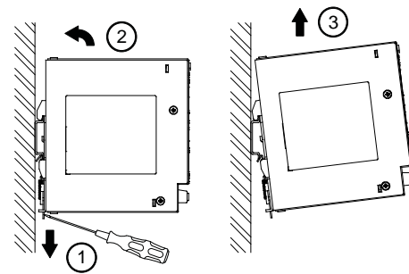
Fig. 6.2 Dismounting
