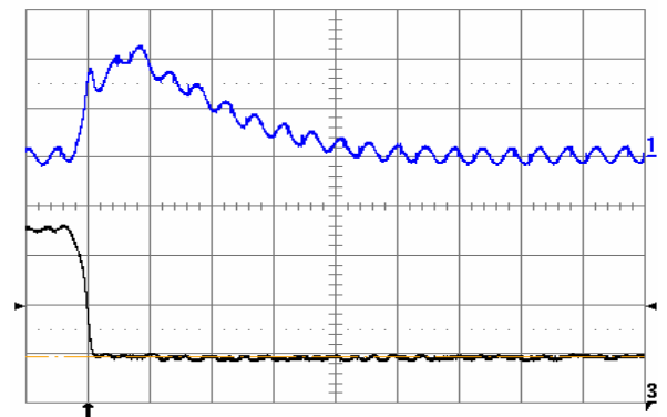
Fig. 10b*: Output voltage response to load current step-change (10 A – 15 A – 10 A) at V_{in} = 48 V. Top trace: output voltage (50 mV/div.). Bottom trace: load current (2 A/div.). Current slew rate: 2.5 A/ \mu s. C_o = 2 \times 100 \mu F TA + 1 \mu F ceramic. Time scale: 5 \mu s/div.
