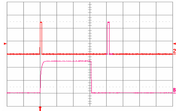
Fig. 16: Load current (top trace, 10 A/div., 50 ms/div.) into a 10 m \Omega short circuit during restart, at V_{in} = 48 V. Bottom trace (10 A/div., 2 ms/div.) is an expansion of the on-time portion of the top trace.
