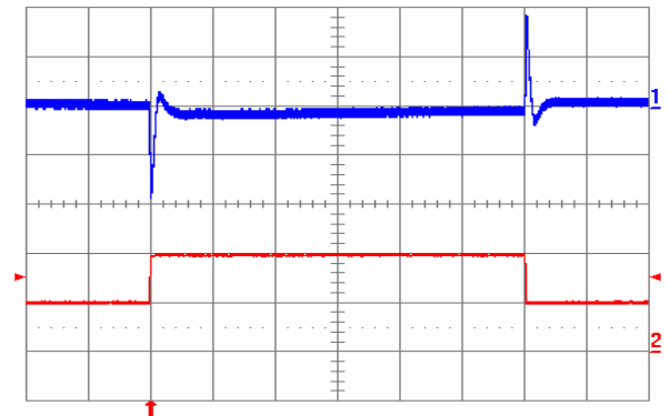
Fig. 10: Output voltage response to load current step-change (10 A – 20 A – 10 A) at V_{in} = 48 V. Top trace: output voltage (100 mV/div.). Bottom trace: load current (10 A/div.). Current slew rate: 5 A/ \mu s. C_o = 470 \mu F POS + 1 \mu F ceramic. Time scale: 0.2 ms/div.
