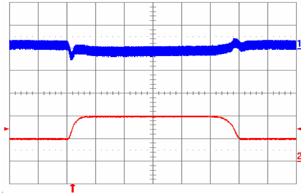
Fig. 9: Output voltage response to load current step-change (10 A – 20 A – 10 A) at V_{in} = 48 V. Top trace: output voltage (100 mV/div.). Bottom trace: load current (10 A/div.). Current slew rate: 0.1 A/ \mu s. C_o = 1 \mu F ceramic. Time scale: 0.2 ms/div.
