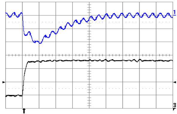
Fig. 10a*: Output voltage response to load current step-change (10 A – 15 A – 10 A) at V_{in} = 48 V. Top trace: output voltage (50 mV/div.). Bottom trace: load current (2 A/div.). Current slew rate: 2.5 A/ \mu s. C_o = 2 \times 100 \mu F TA + 1 \mu F ceramic. Time scale: 5 \mu s/div.
