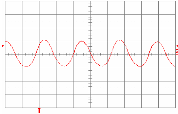
Fig. 13: Input reflected ripple current, i_c (100 mA/div.), measured at input terminals at full rated load current and V_{in} = 48 V. Refer to Fig. 12 for test setup. Time scale: 1 \mu s/div.
