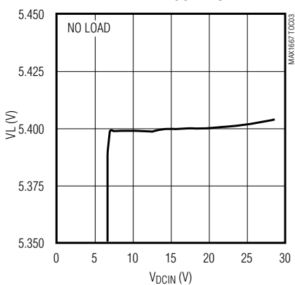
VL LINE REGULATION
