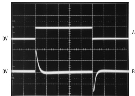
MAX6125 LINE-TRANSIENT RESPONSE
