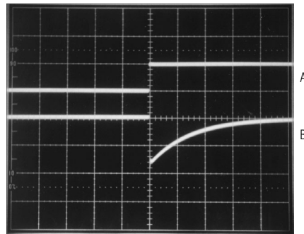
MAX6125 LOAD-TRANSIENT RESPONSE (SOURCING)
