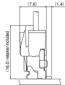
PA Receptacle (Retainer mountable type) + PA Header
