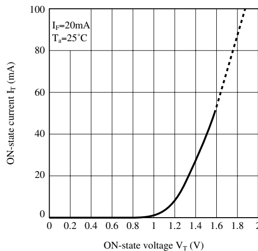
Fig.12 ON-state Current vs. ON-state Voltage
