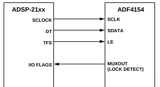
Figure 25. ADSP-21xx to ADF4154 Interface
