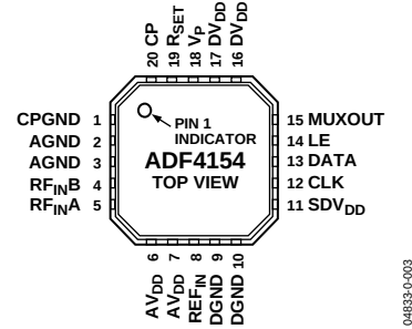
Figure 4. LFCSP Pin Configuration
