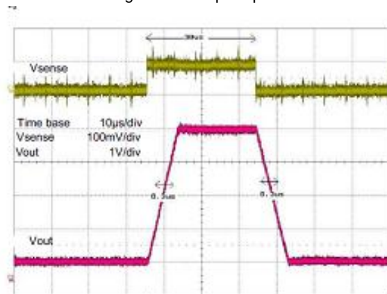
Figure 12: Step response
