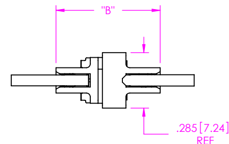
FIGURE 4 QSE-XX-EMX MATED WITH QTE-XX-EMX
