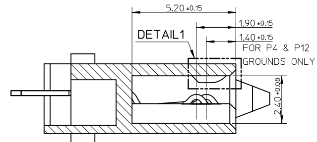
SECTION Z-Z
