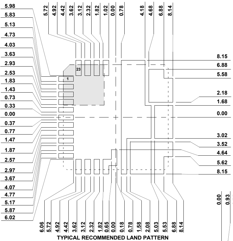
TYPICAL RECOMMENDED LAND PATTERN
