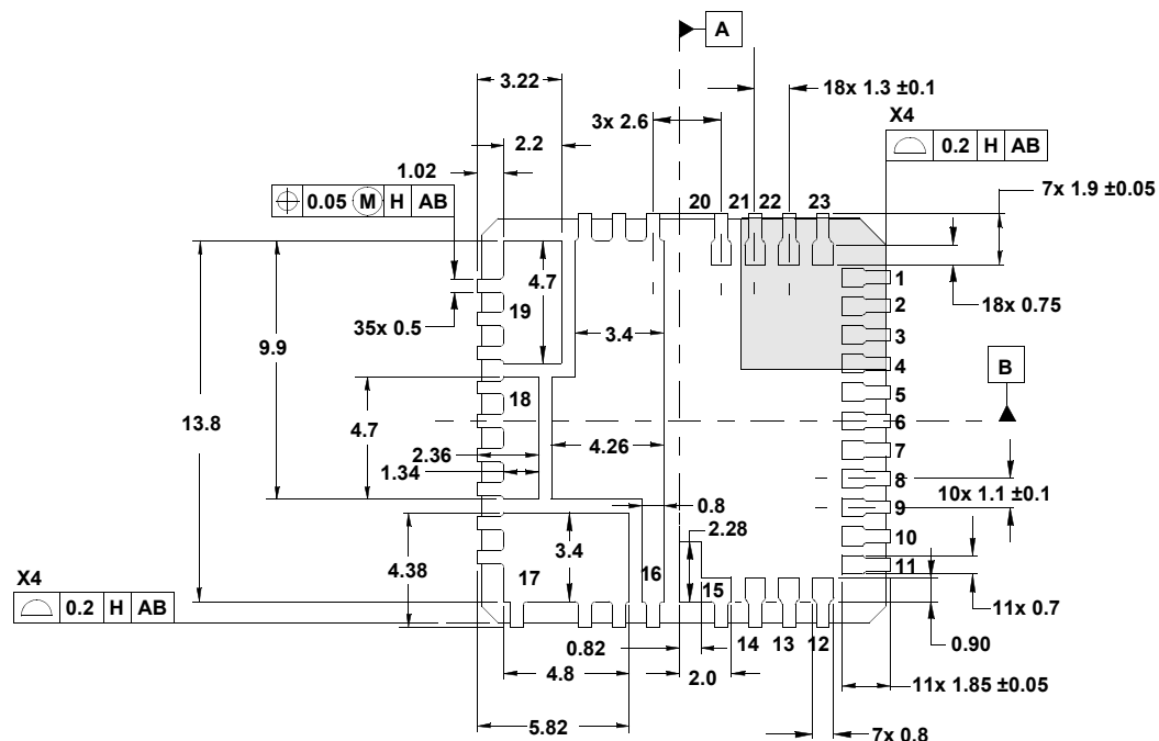
BOTTOM VIEW
