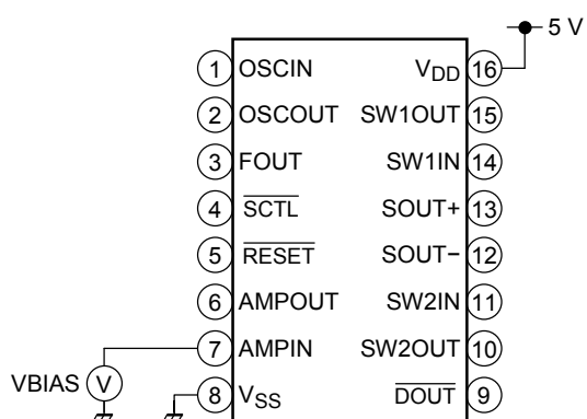
(17) Amplifier input bias voltage
