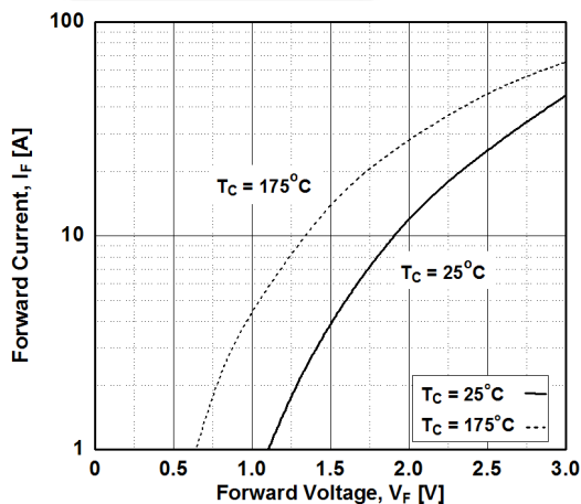
Figure 17. Forward Characteristics
