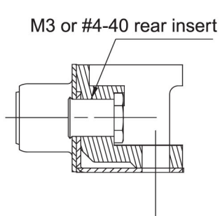
Threaded Rear
