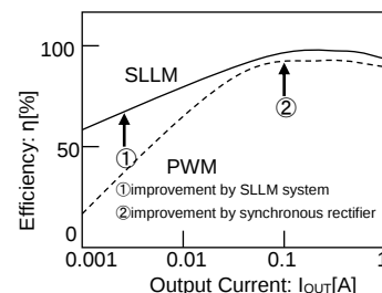
Figure 25. Efficiency
