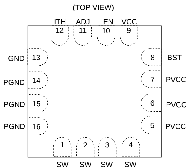
Figure 2. Pin Configuration
