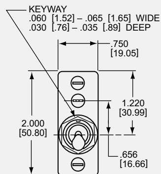
Single Pole
