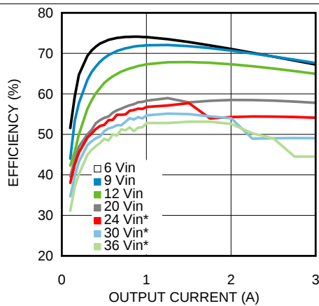
Figure 13. Efficiency 1.2-V Output at 25°C Ambient
