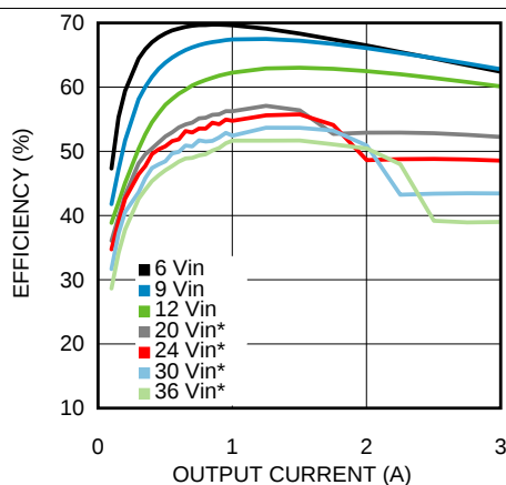
Figure 15. Efficiency 1-V Output at 25°C Ambient
