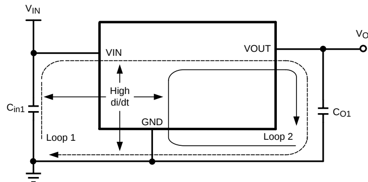
Figure 54. Critical Current Loops to Minimize
