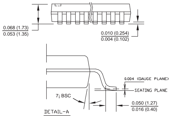
20-Pin QSOP (QS)
